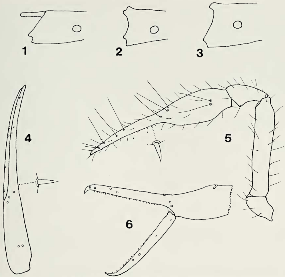
Figures 1-6.—Species of Kleptochthonius . 1-3. Proximal end of movable finger of palpal chela, lateral view, showing dorsal process (dorsal at top; areole is that of trichobothrium b ). 1. Kleptochthonius packardi , lectotype male; 2. Kleptochthonius griseomanus new species, holotype female; 3. Kleptochthonius lewisorum new species, holotype female. 4. Kleptochthonius packardi , lectotype male: Left palpal chela, dorsal view, with enlargement of sensory seta on fixed finger (other setae omitted). 5, 6. Kleptochthonius griseomanus new species, holotype female. 5. Right palp, dorsal view, with enlargement of sensory seta on fixed finger; 6. Left chela, lateral view (base broken; setae omitted).
